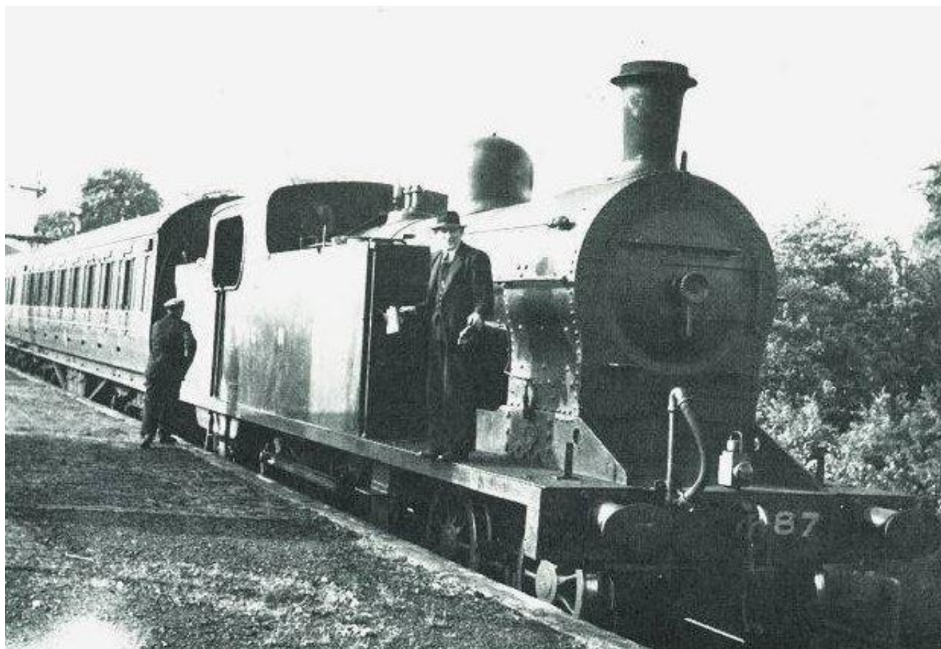
T1 No.187 at Drumsough on 16 th May 1952. The train was the 5:38pm ex York Road, all stations to Drumsough, returning immediately. Loco Inspector W. Hanley stands on the running plate. (A. Donaldson)
